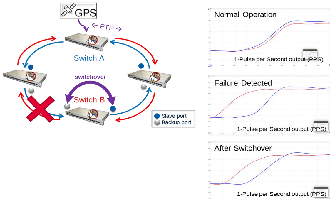
Figure 2. Scheme of robust linked clocks
